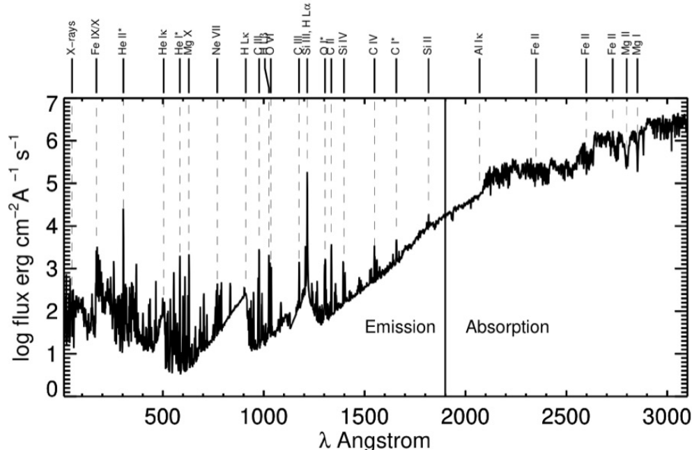
Figure 1. The solar flux spectrum as measured on Mar 25-29 2008 with various instruments, compiled by staff at LASP as part of the Whole Heliospheric Interval Campaign, from http://lasp.colorado.edu/lisird/ . The spectrum is from soft X-rays to near the atmospheric cut-off, highlighting emission and absorption features. The region has a number of deep absorption lines with emission in their core. Mg II is such an example, although the emission is not observable due to the modest spectral resolution. The transitions of H, He I and He II, with \Delta n = 1 and are labeled with asterisks are compared with \Delta n = 0 transitions of much more highly ionized species at similar wavelengths.
